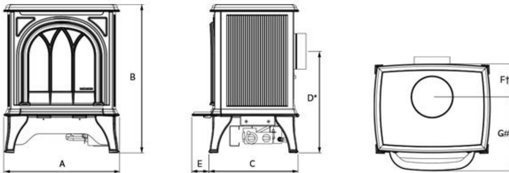
Huntingdon 20 Dimensions (see letters on diagram)
